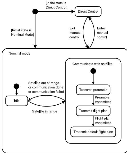
Fig. 6. State diagram of overall states.
