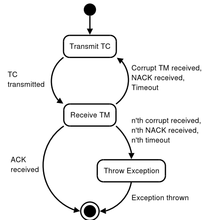
Fig. 5. State diagram for retransmission.
