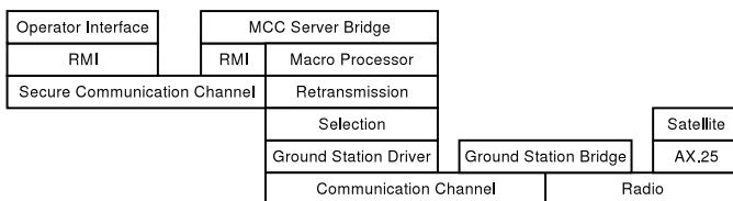
Fig. 8. Protocol stack for communication with the satellite.
