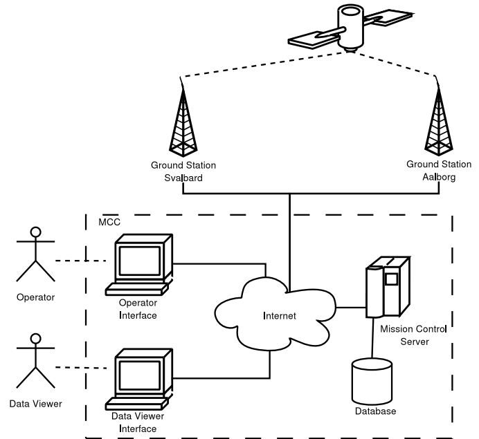
Fig. 2. Overall structure of the MCC.
