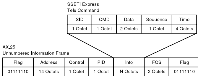
Fig. 3. AX.25 encapsulation of a SSETI Express tele command.
